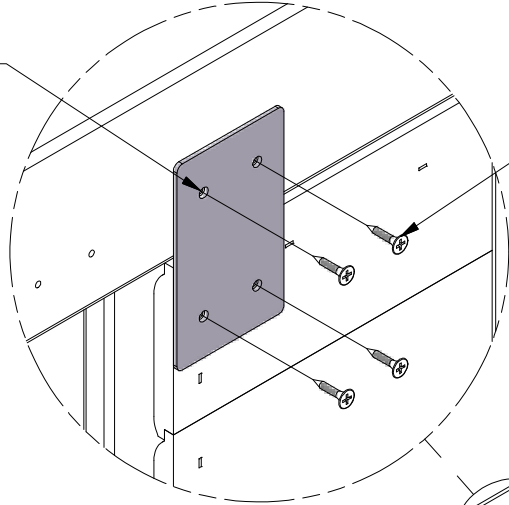
395 (x32) SCREW - 3/4"
