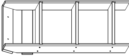
(x1) LADDER SUBASSEMBLY
