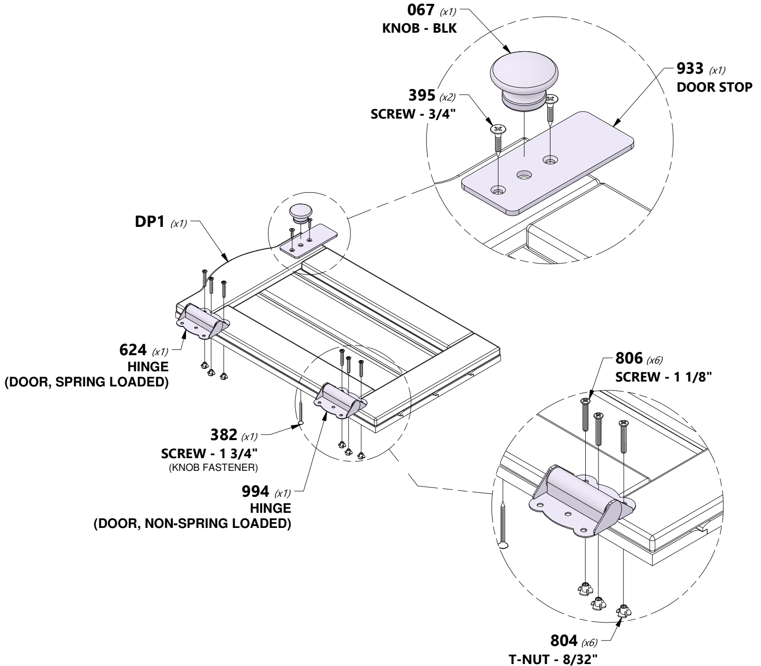
A4M00994 (x1) HINGE (DOOR, NON-SPRING LOADED)
