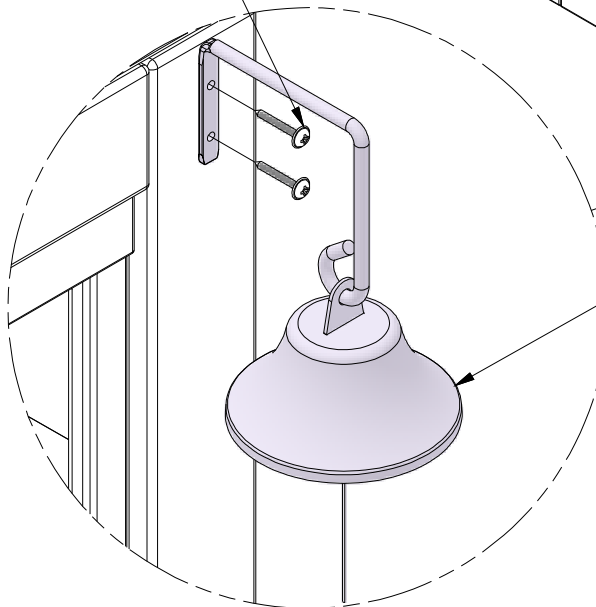
797 (x2) SCREW - 1"
