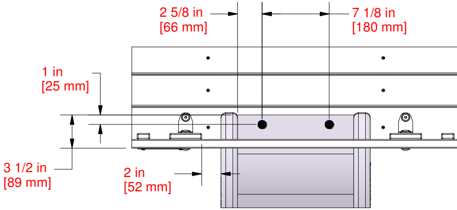
DRILLING LOCATIONS
